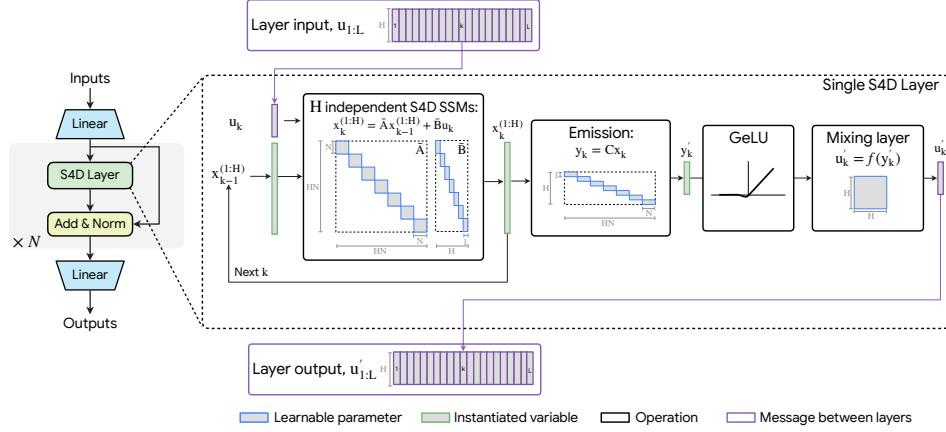
Figure 2.2: S4D Encoder structure. Inspired by the visualization in [16], the input of dimension H is processed by H parallel SSMs. For non-linearity, GeLU [39] is employed. Mixing layer is applied to mix outputs from these H SSMs.
