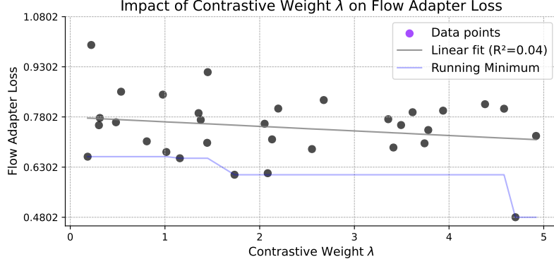
Figure 3.5: Flow adapter loss w.r.t contrastive weight.
