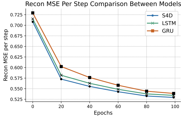
Figure 2.4: Comparison between sequence models: reconstruction MSE for the skill latent model using different building blocks (LSTM, GRU, and S4D).
