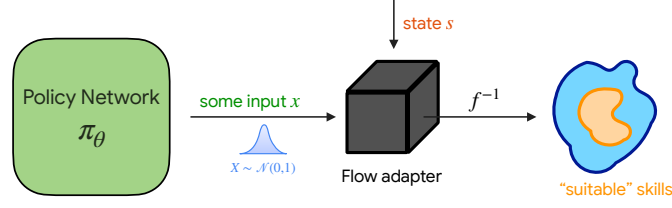
Figure 3.2: Design of flow adapter: input with simple distribution is then transformed to a complex distribution conditioned on the partial-state signal.
