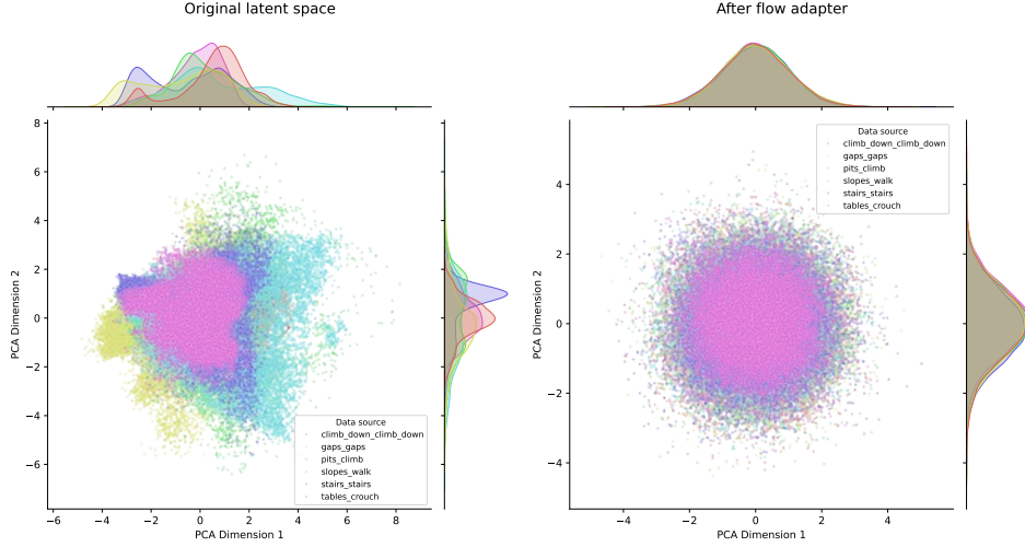
Figure 3.6: Visualization of the skill latent space using PCA. Left: original skill latent space; Right: skill latent space after flow adapter transformation: y = f(z, s) , here z and s are taking in pairs, which means latent vector is produced by the skill action a with the encoder of skill latent model, and z is the corresponding partial state of a .
