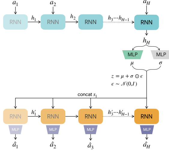
Figure 2.1: Structure of skill latent encoder-decoder. From left to right means time unrolling direction
