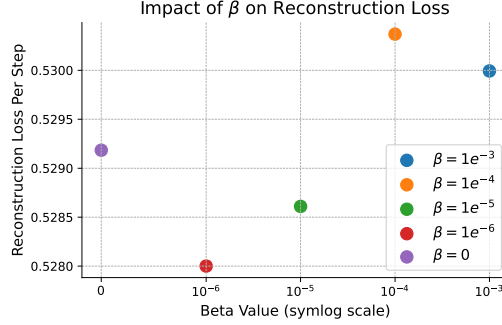
Figure 2.7: Comparison of reconstruction MSE per step across different values of \beta , which controls the strength of the KL regularization in the latent space. As \beta increases, the latent space is increasingly constrained towards a Gaussian prior, influencing the model’s reconstruction quality. The results indicate that small values of \beta slightly improve or maintain performance compared to the unregularized model, while larger values do not provide significant benefits, \beta value larger than 1 tend to affect the reconstruction quality significantly.
