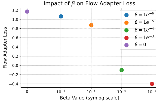
Figure 3.4: Flow adapter loss w.r.t \beta values.
