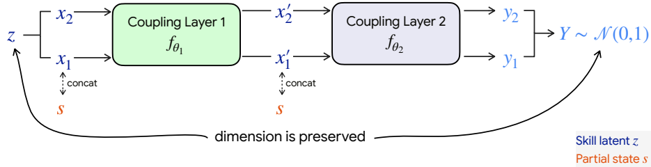
Figure 3.1: An example of a partial state-conditioned flow adapter with two coupling layers parameterized by \theta_1 and \theta_2 , respectively. The input is first split into two vectors, x_1 and x_2 , and then processed through two affine coupling layers.
