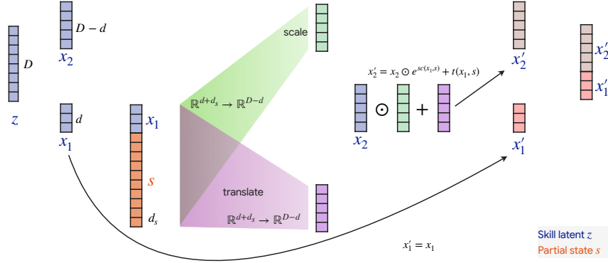
Figure 3.3: Implementation of coupling layer with partial state information as conditioning, in our implementation we use random permutation for breaking up the input vector z .
