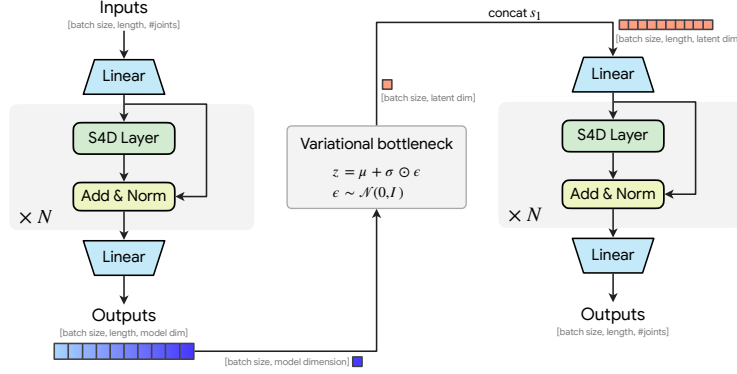
Figure 2.3: Skill Latent Encoder-Decoder Structure with S4D. The encoder and decoder share the same structure, where the encoder only takes the last step output before feeding it into the variational bottleneck. The decoder takes the entire output as input, with the latent vector duplicated along the sequence length dimension and concatenated with the state.
