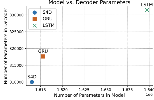
Figure 2.5: Comparison of parameter efficiency between sequence models for the skill latent model and decoder. The S4D model demonstrates superior parameter efficiency compared to GRU and LSTM, using fewer parameters while maintaining or slightly improving performance.
