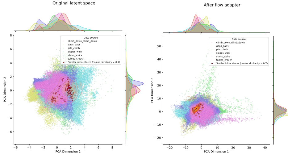
Figure 4.11: Visualization of the skill latent space using PCA. Left: original skill latent space; Right: latent space after applying the flow adapter. The flow adapter creates a more structured latent space, making it easier for the policy to explore relevant actions.
