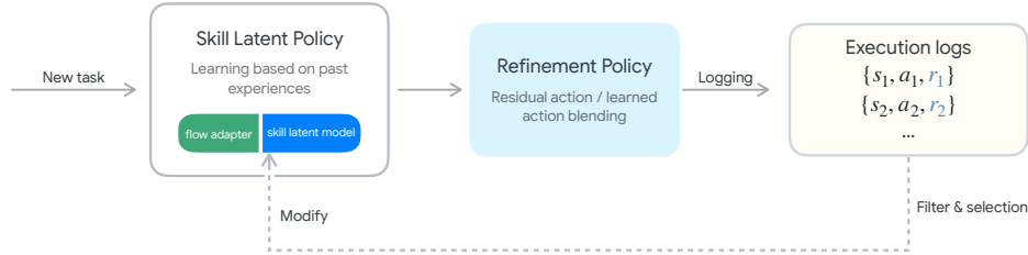
Figure 1.1: The continuous skill learning framework consists of three components: a skill latent policy that learns from past experiences, a refinement policy that adapts the skill latent policy’s output to the current environment, and a periodic log memory for storing execution logs that may be useful for future learning.
