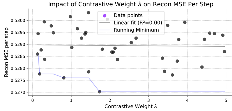
Figure 2.9: Reconstruction MSE per step as a function of contrastive weight \lambda . The results suggest that there is no strong correlation between the contrastive weight and reconstruction quality. Moderate contrastive regularization does not significantly affect the decoder's ability to reconstruct the data.
