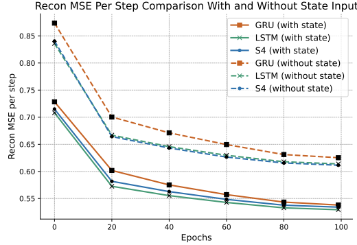
Figure 2.6: Impact of initial state information: Reconstruction MSE per step comparison with and without the initial state s_1 as input to the skill latent decoder.
