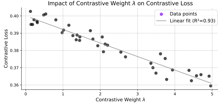
Figure 2.8: Contrastive loss as a function of the contrastive weight \lambda . As \lambda increases, the contrastive loss decreases, reflecting the increased focus on representation alignment in the latent space.
